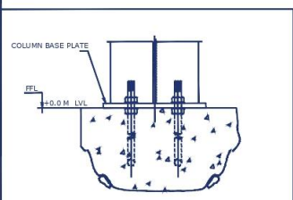
SECTIONAL VIEW - 2 BOLTS IN A ROW
